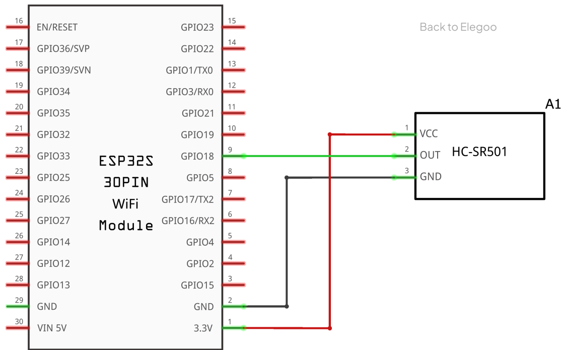
Wiring diagram
